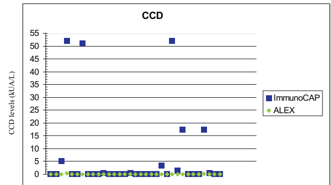
Fig. 2. CCD detection in pollen allergy with ImmunoCAP® and ALEX®.
